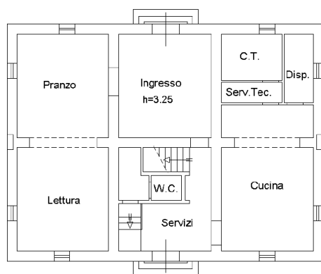
PIANO TERRA
